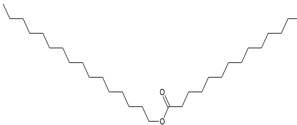
Hexadecanoic acid, hexadecyl ester
